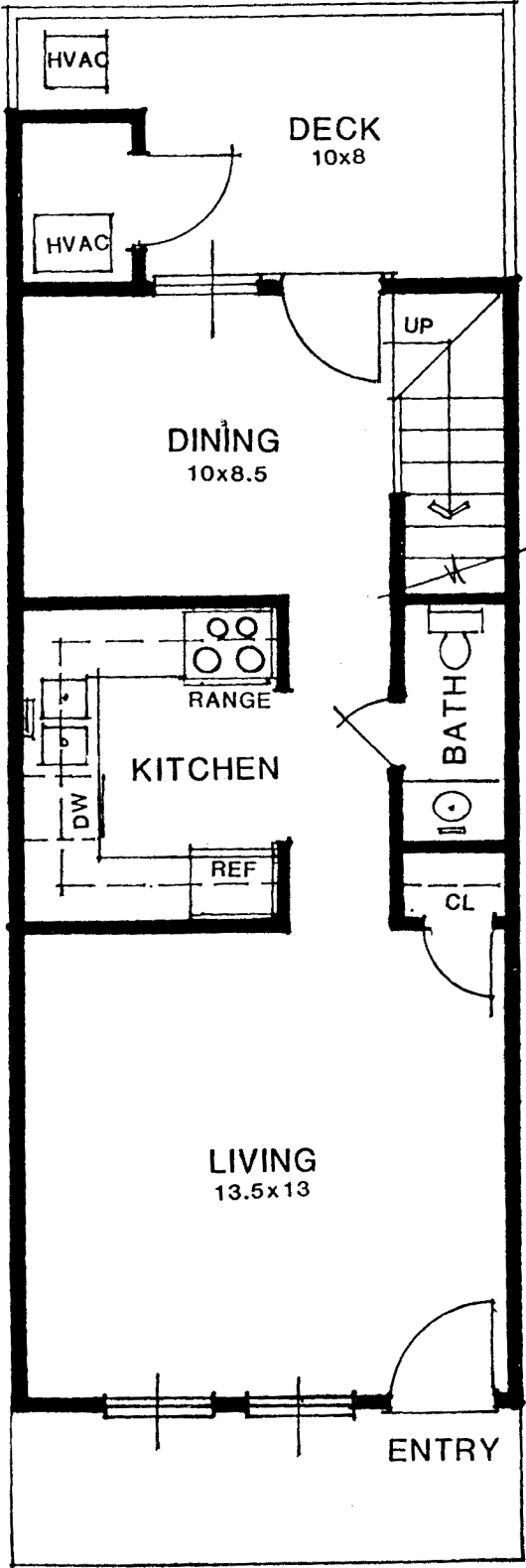
FIRST FLOOR
