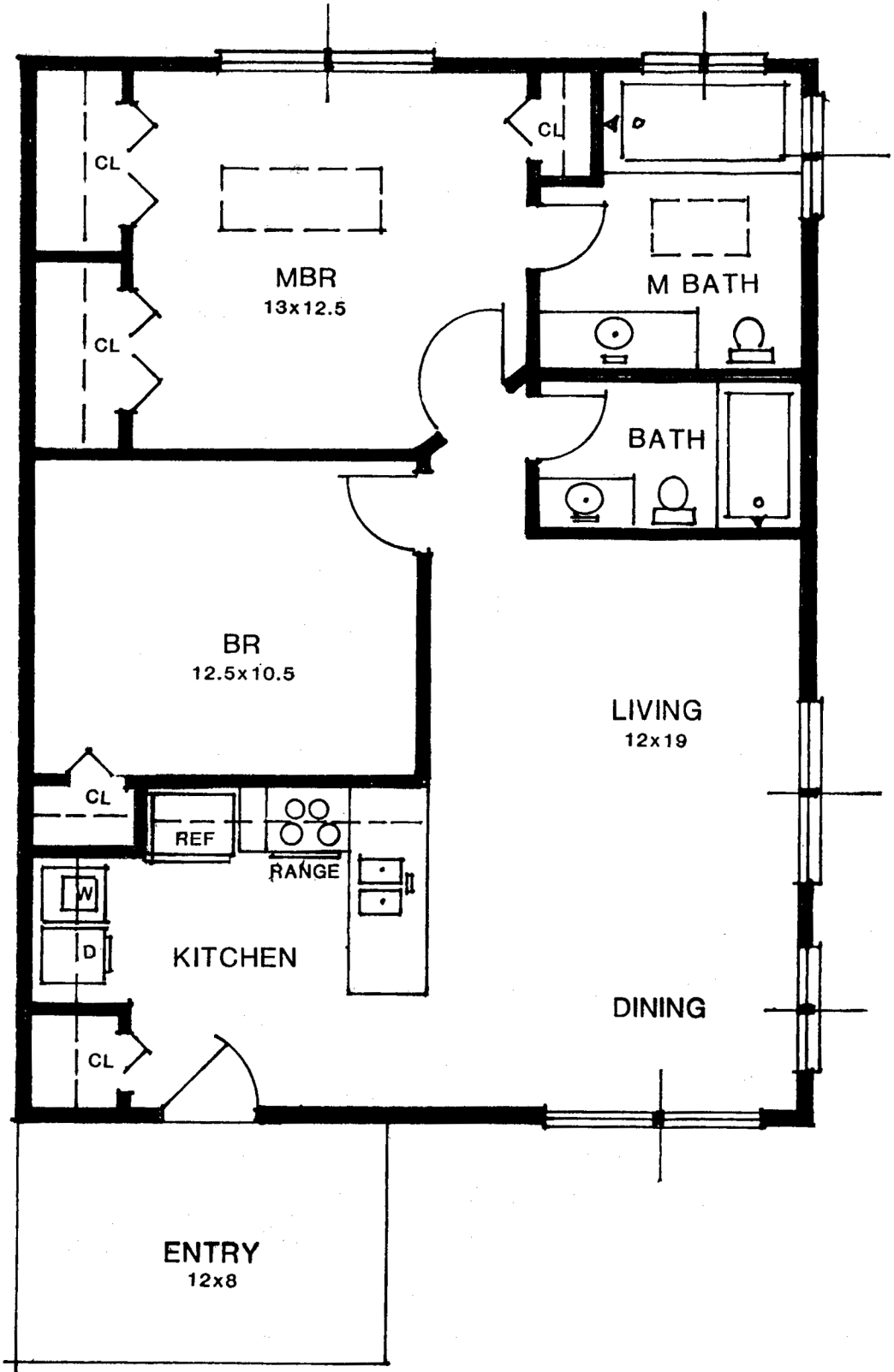
FLOOR PLAN
